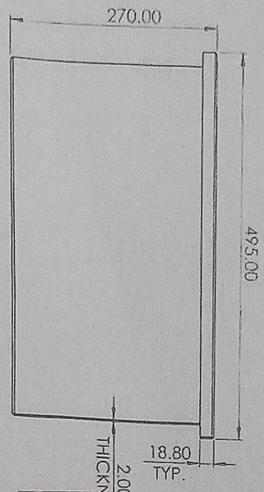
FRONT VIEW
