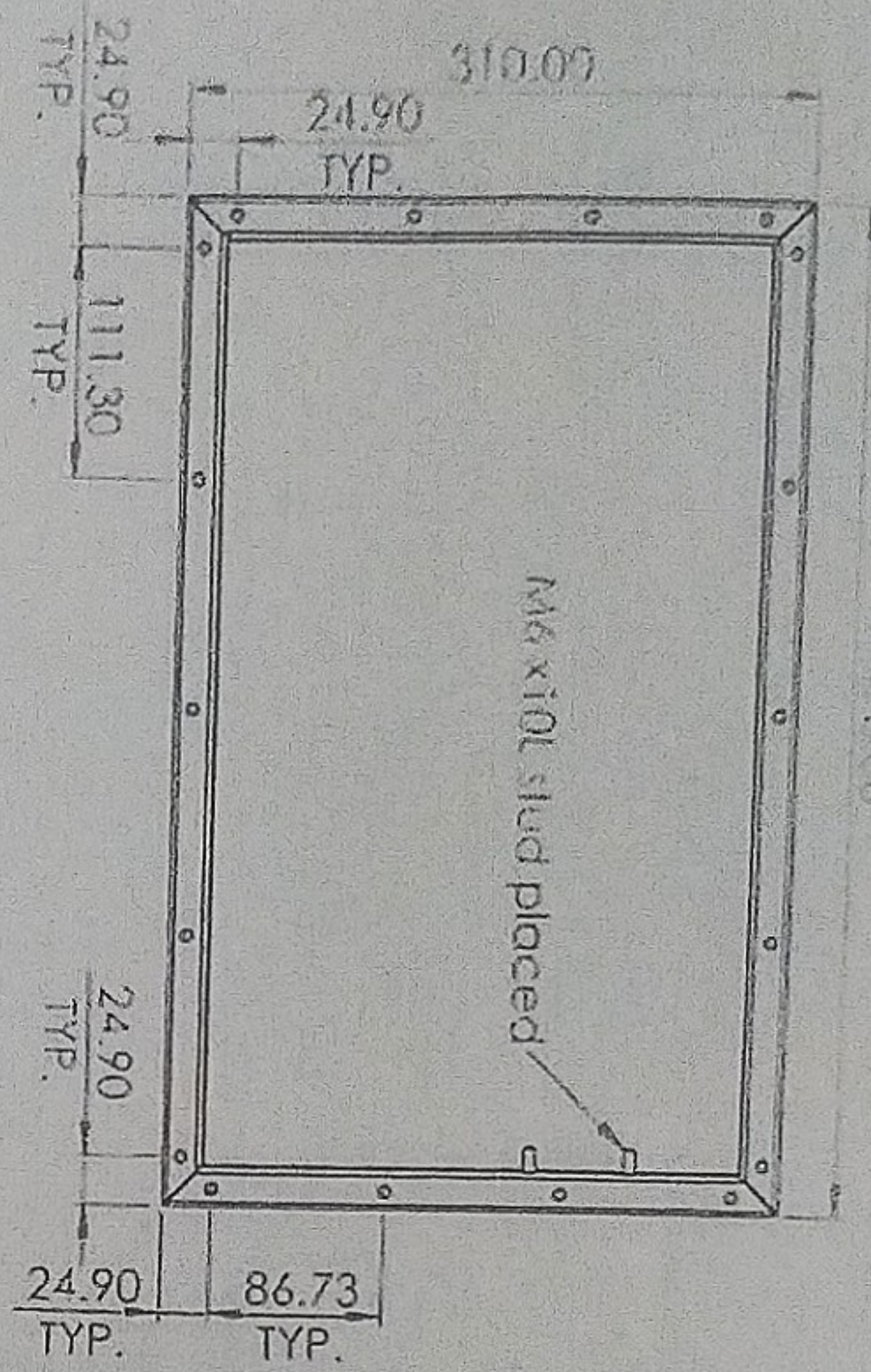
TOP VIEW
